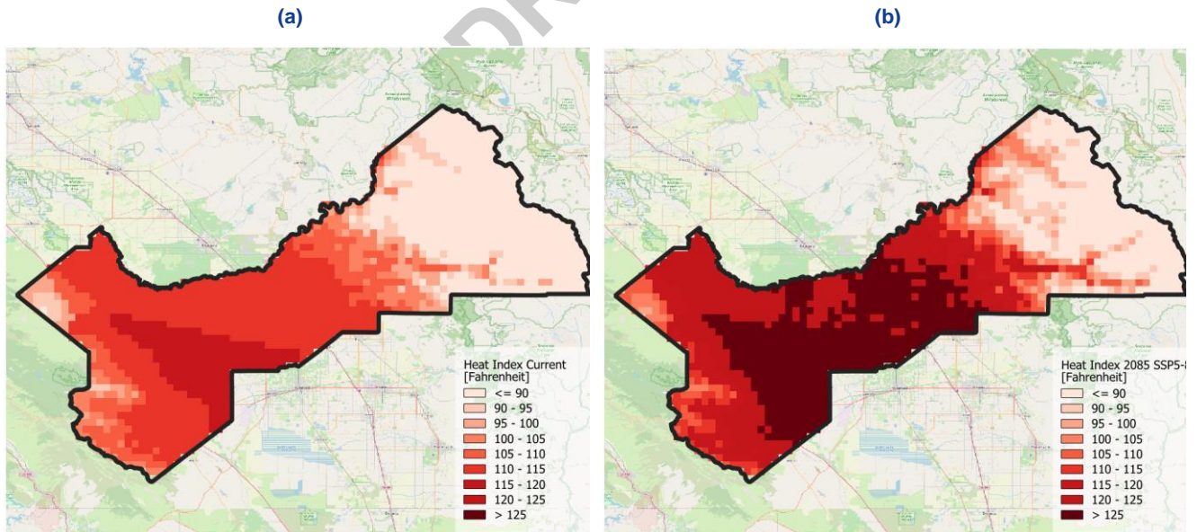
Figure 2-4. Extreme annual heat index for 1 in 5-year extreme heat event for (a) present-day climate and (b) end of century climate, SSP5-8.5 2085.
