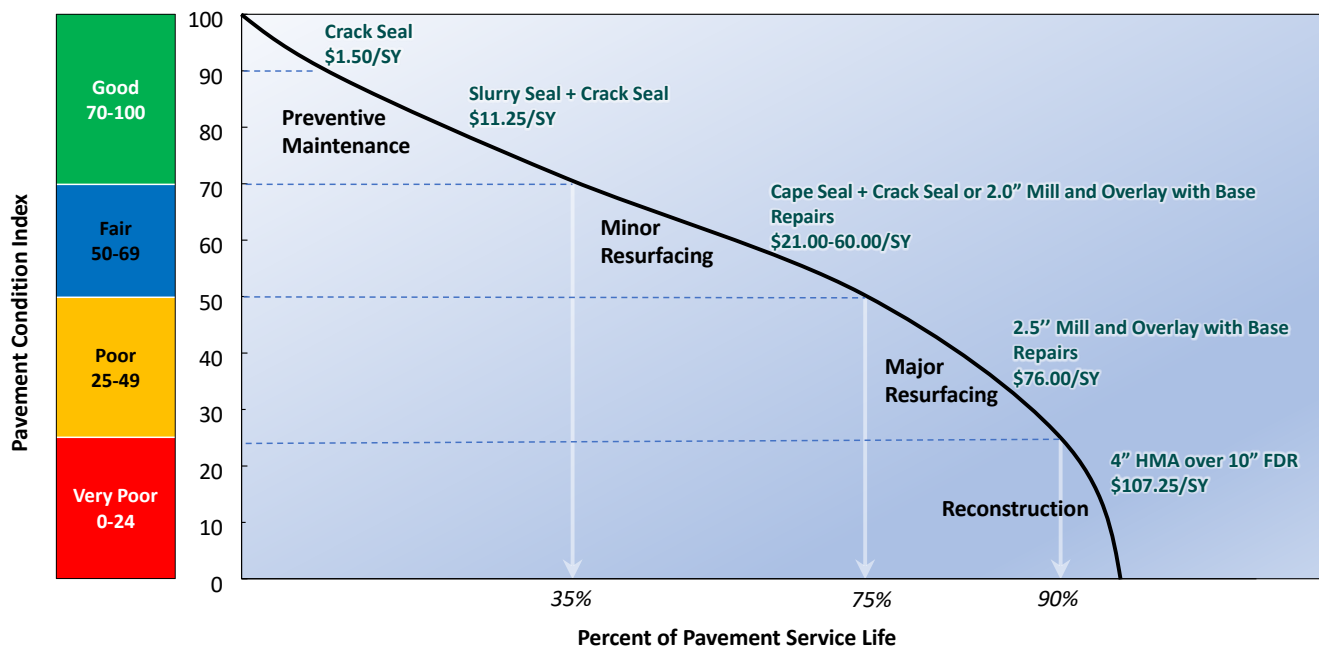
Figure 5. Costs 5 of Maintaining Arterial over Service Life.
