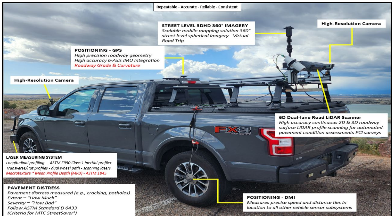
Figure 1. NCE's Data Collection Vehicle.
