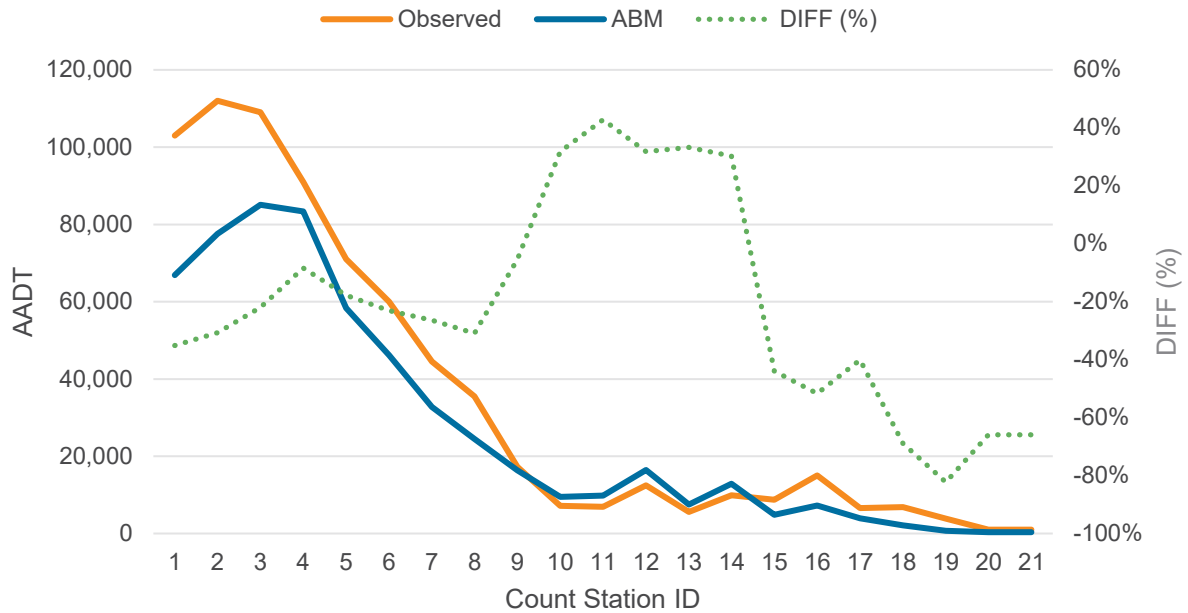
FIGURE 28: HIGHWAY VALIDATION – SR168 (WEST TO EAST)
